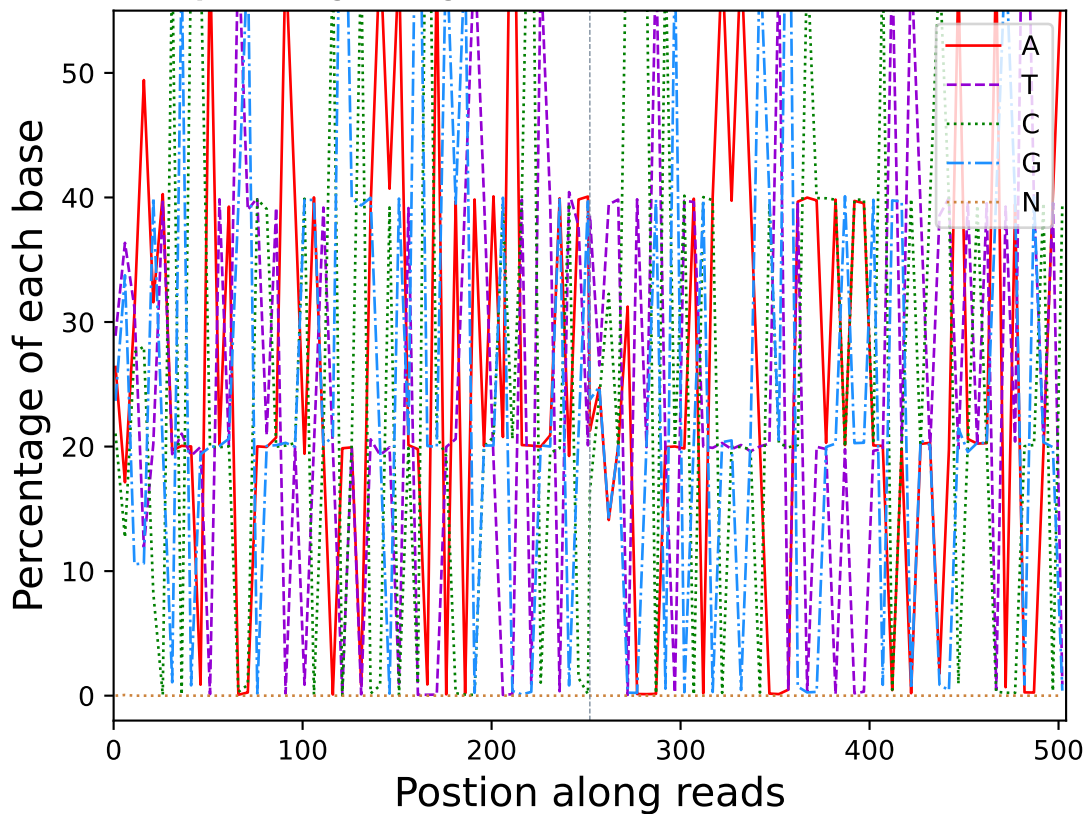
Base percentage along reads (R10608)
